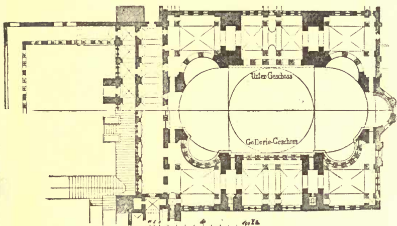
GROUND-PLAN OF THE CHURCH OF S. SOPHIA
